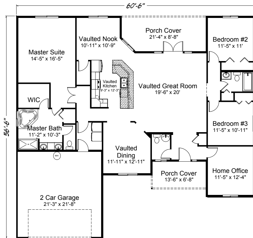
Harbor Point 2168 sq. ft. • 3 Bedrooms 2.5 Baths 2 car garage
